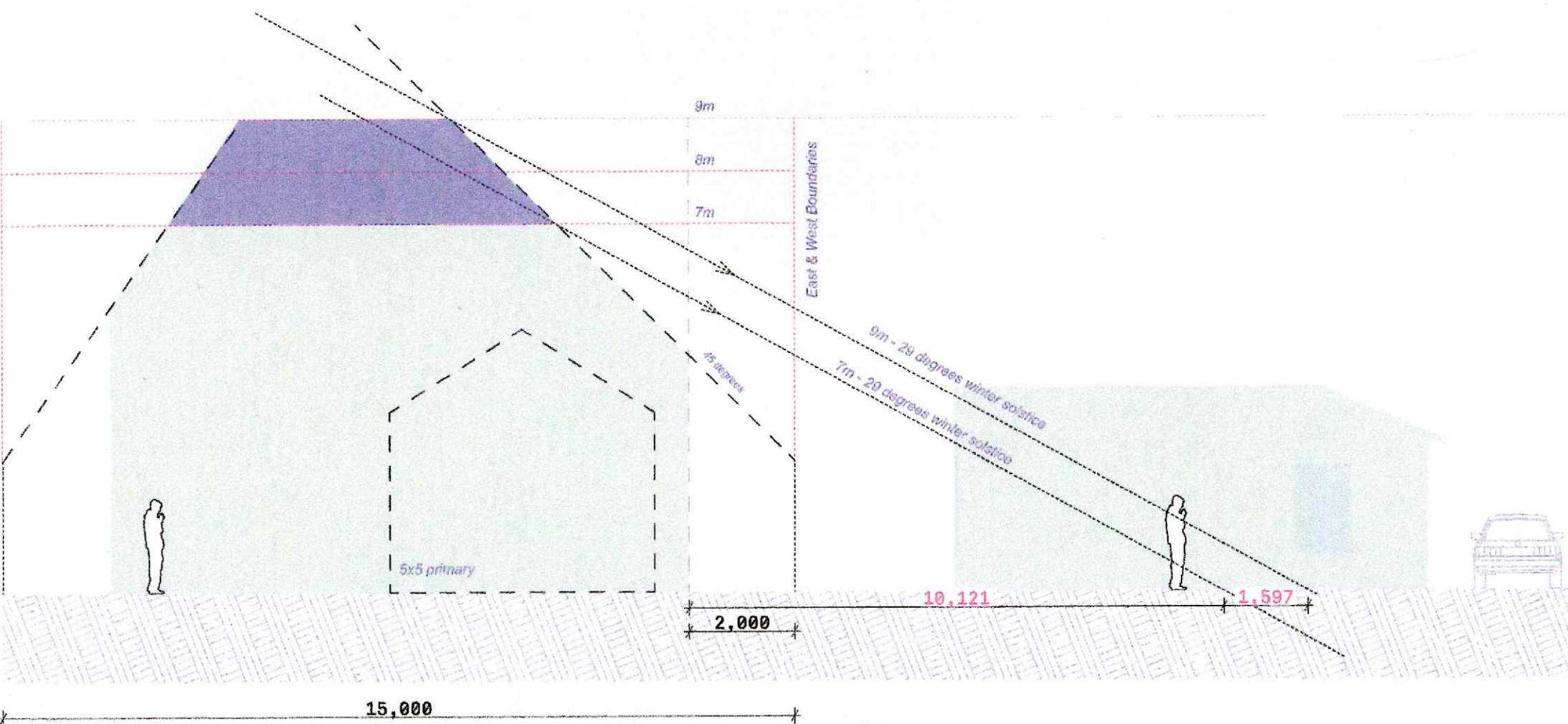
SHADING CAST BY INCREASE IN HEIGHT - PERMITTED BASELINE - WINTER SOLSTICE
