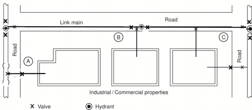
Figure 6.3 – Secure connection
