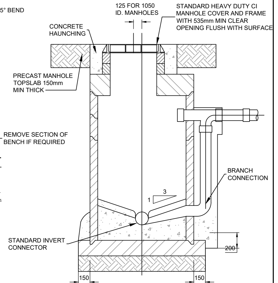
SECTION - EXTERNAL DROP MANHOLE
