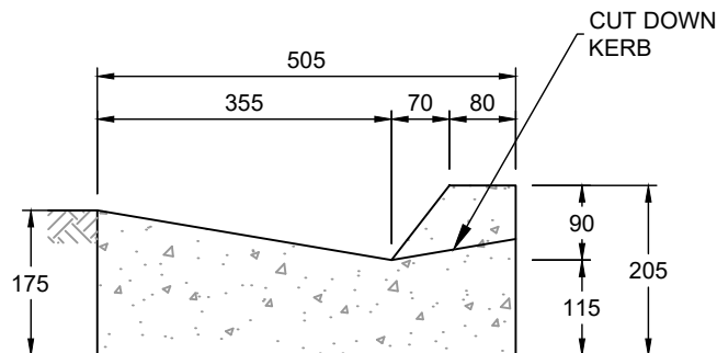
No. 8 MOUNTABLE KERB & CHANNEL
