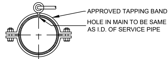
SECTION A
