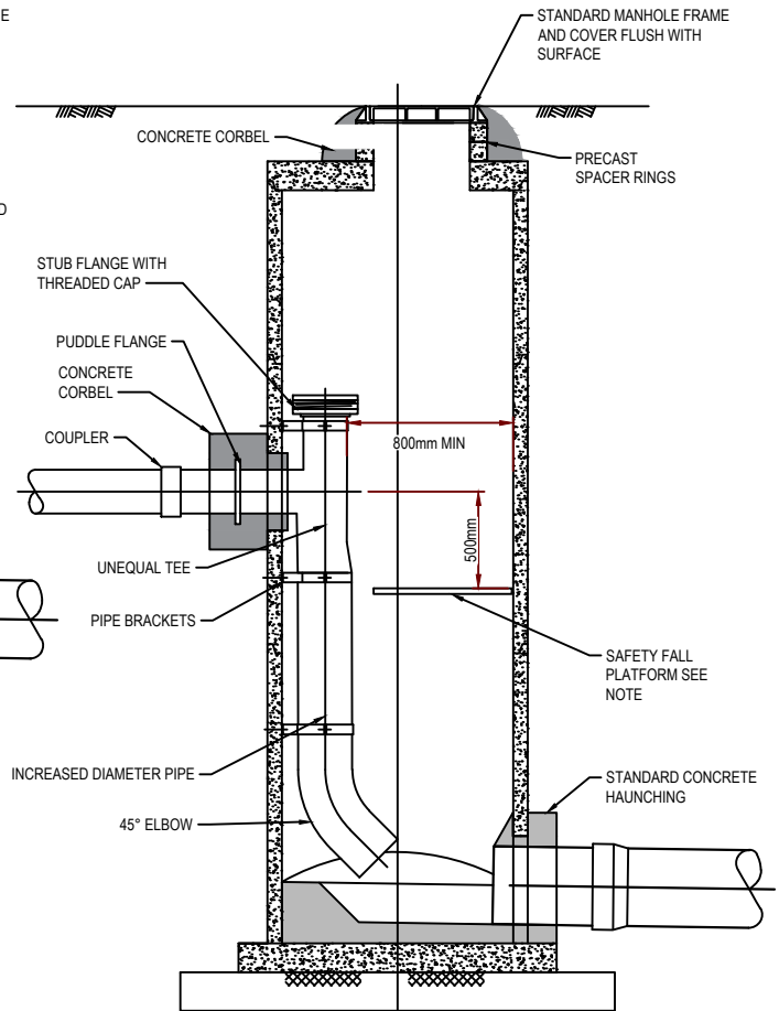
SECTION B-B' IF DROP STRUCTURE IS REQUIRED
