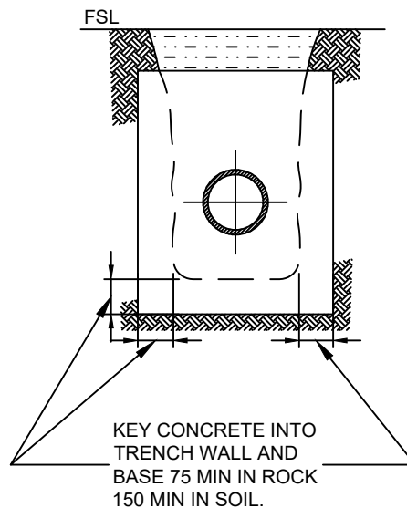
SECTION A
