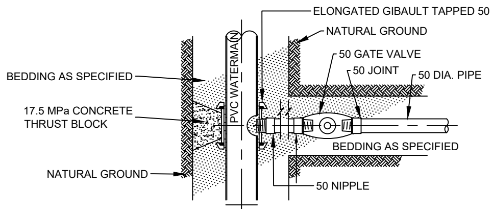
90° CONNECTION - PLAN RIDER MAIN CONNECTIONS
