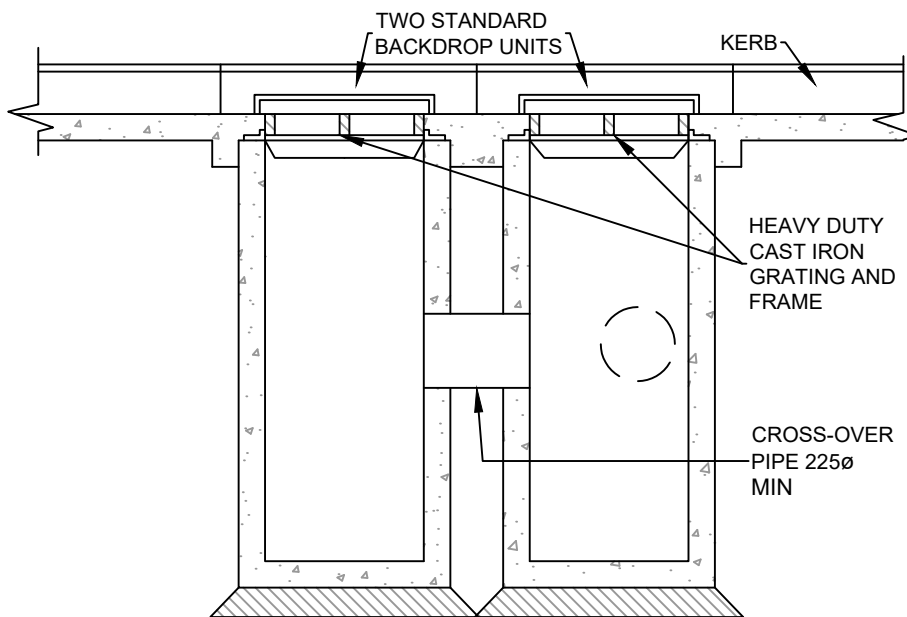
SECTION B
