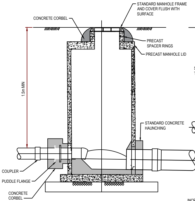
SECTION B-B' FOR SHALLOW CIRCULAR PRECAST MANHOLES
