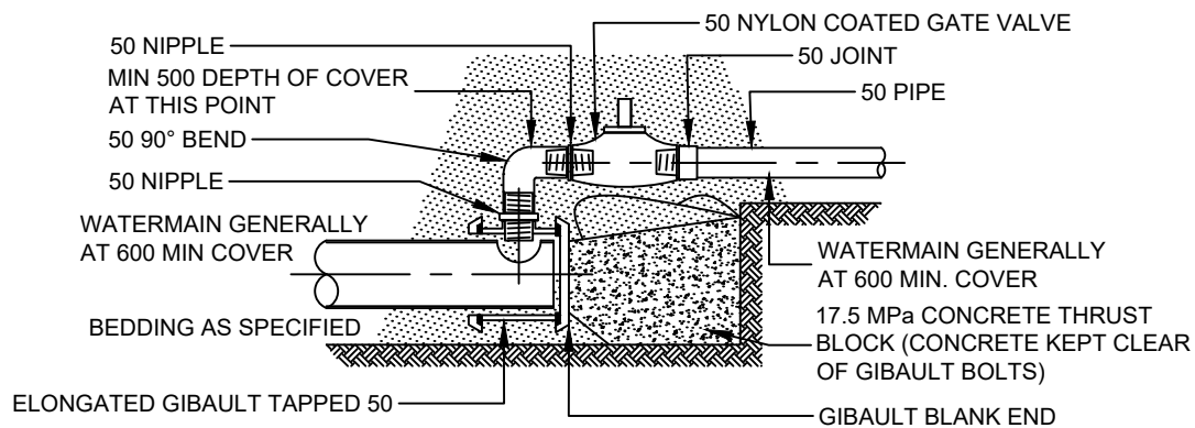
STRAIGHT LINE CONNECTION - METHOD 1 - ELEVATION
