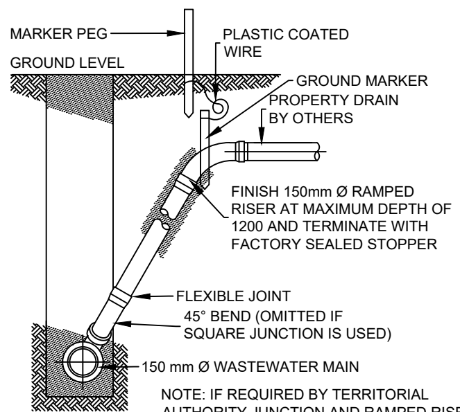
ELEVATION Y JUNCTION RAMPED RISERS
