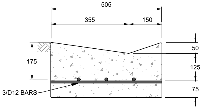
No. 2A COMMERCIAL VEHICLE CROSSING
