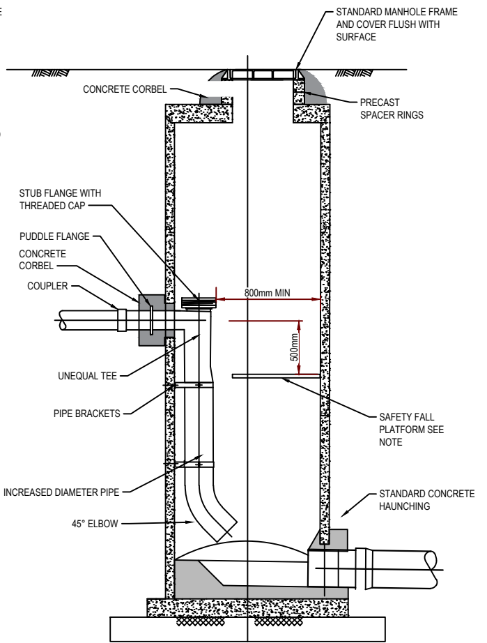
SECTION A-A' IF DROP STRUCTURE IS REQUIRED
