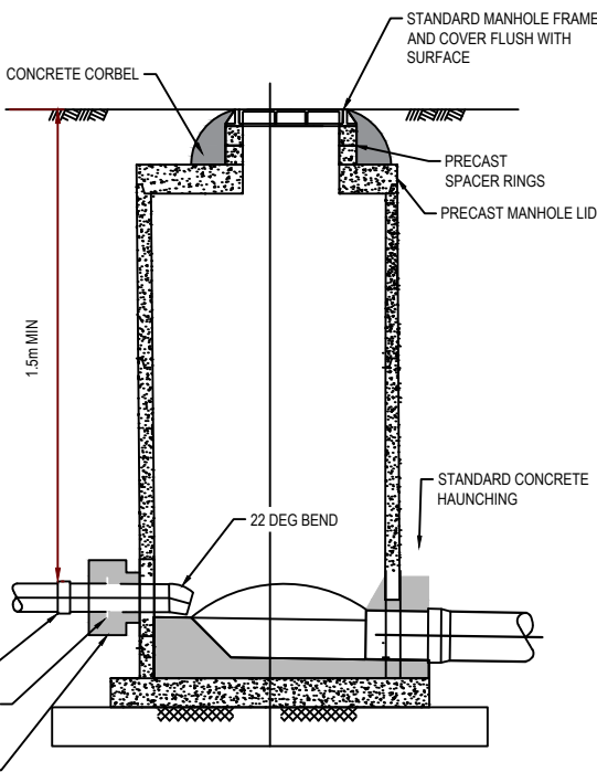
SECTION A-A' FOR SHALLOW MANHOLES
