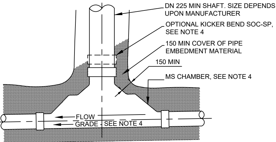
END ELEVATION MAINTENANCE SHAFT
