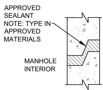
TYPICAL JOINT DETAIL
